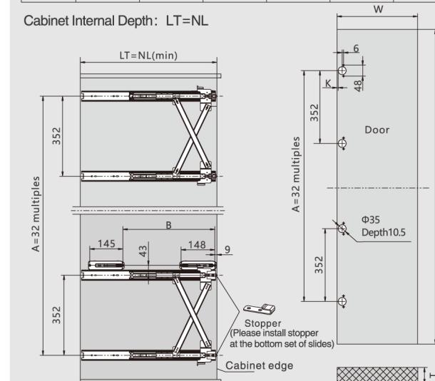
Two sets of slides's installation dimensions
