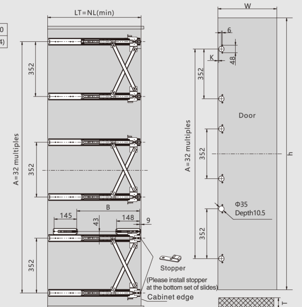
Three sets of slides's installation dimensions
